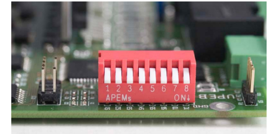
Fig 15: TM44 Dipswitches
