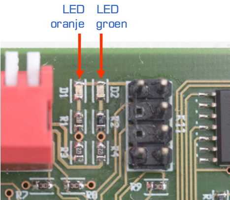
Fig 16: TM44 LEDs
