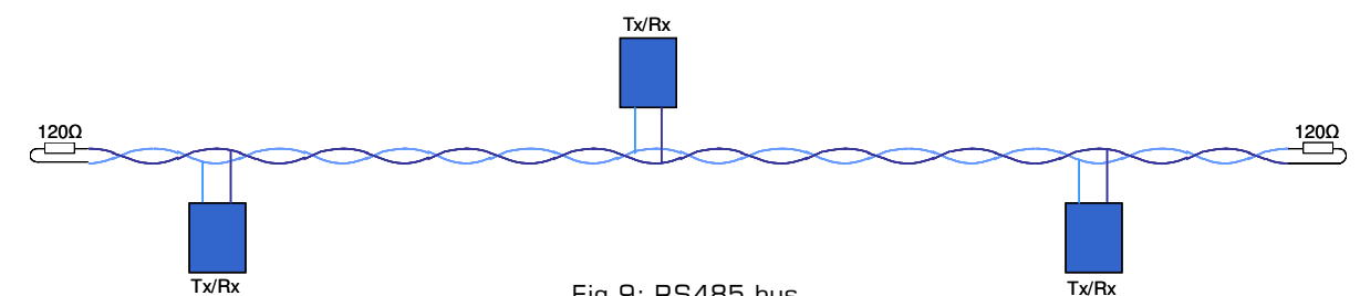
Fig 9: RS485 bus
